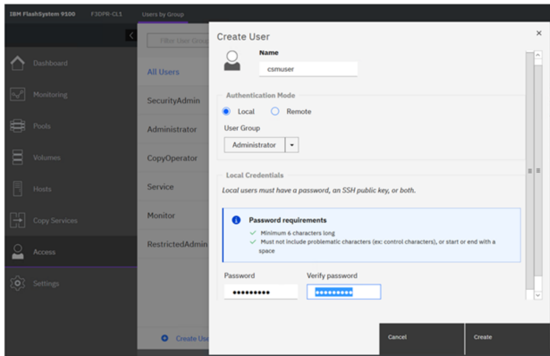
Figure 3-8 Creating an Administrator user
