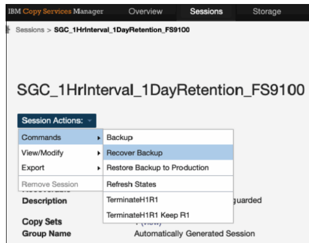
Figure 4-1 Session Actions using Recover Backup
