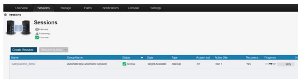
Figure 3-10 Safeguarded Copy session automatically visible in IBM Copy Services Manager
