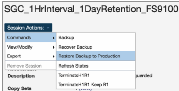
Figure 4-19 Key command difference to restore backup to production
