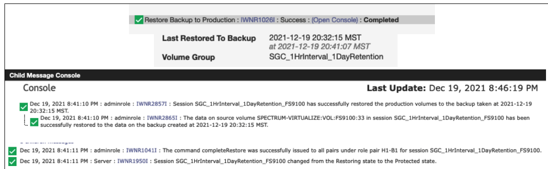
Figure 4-21 Recover Backup to production confirmations
