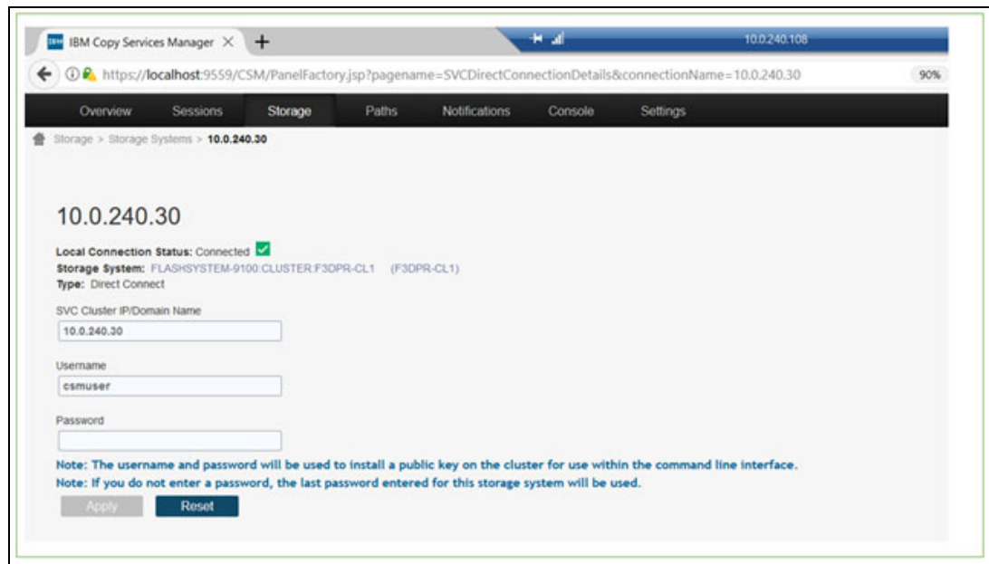
Figure 3-9 Create a connection to the system in the IBM Copy Services Manager interface
