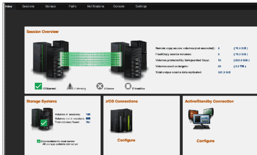
Figure 4-16 Copy Services Manager main screen
