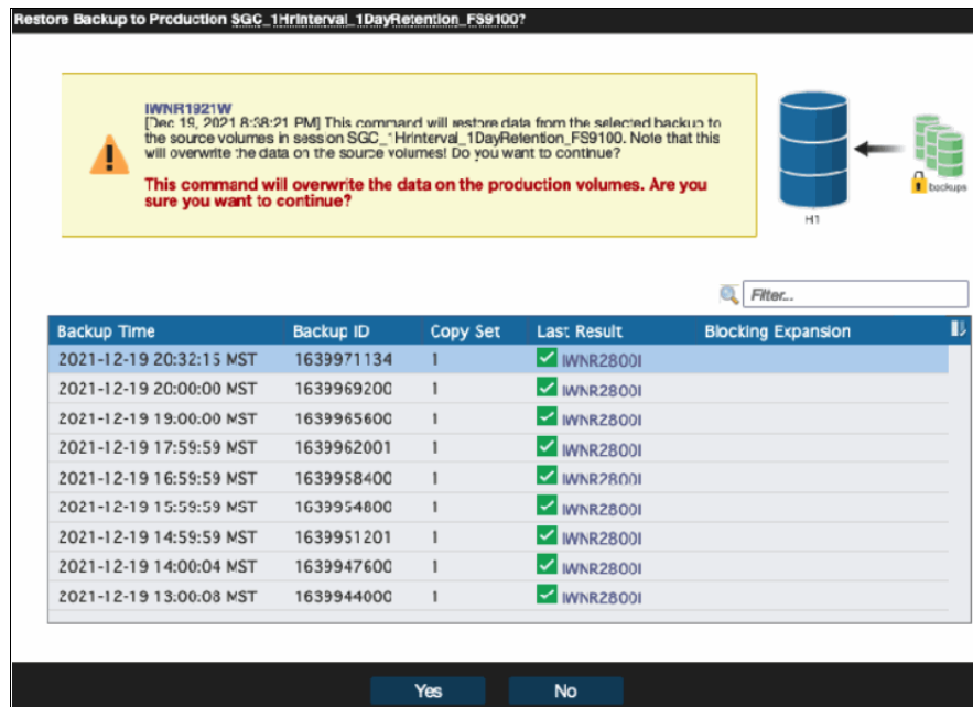
Figure 4-20 Select the specific Safeguarded Snapshot to restore to existing host
