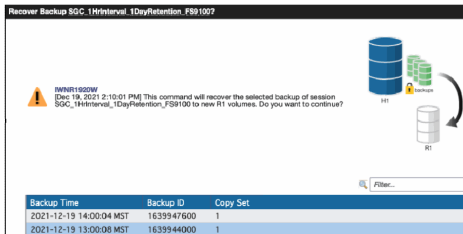
Figure 4-6 Select the specific Safeguarded snapshot to recover to a new host
